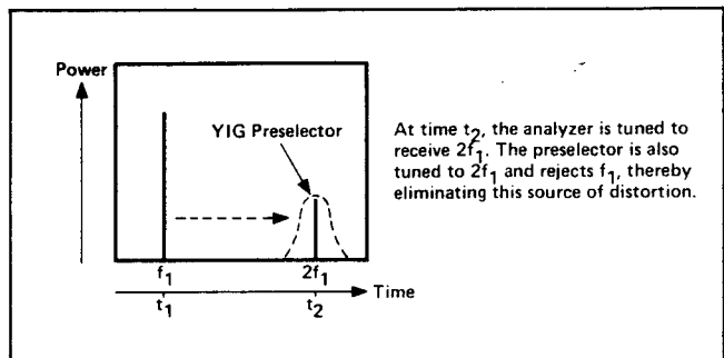
Figure 15. YIG preselector tuning
